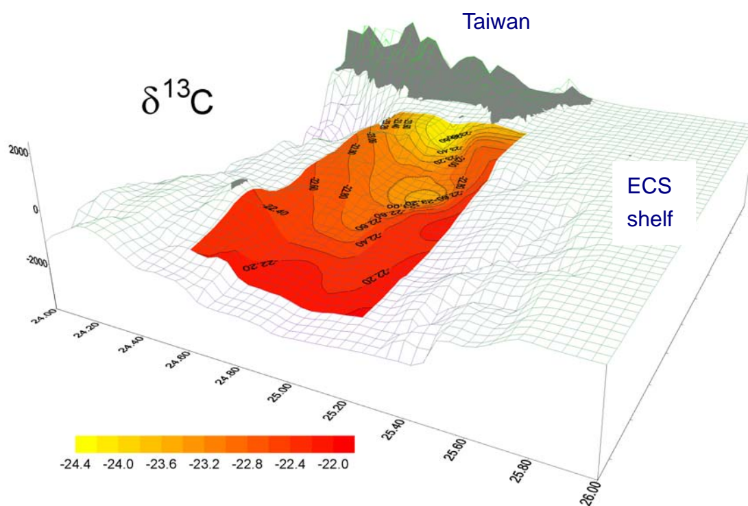
Distribution of grain size and \delta^{13}\text{C} in surficial sediments of southern Okinawa Trough
