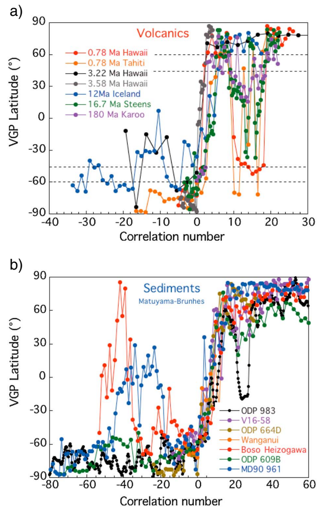
Figure 13. (a) Stratigraphic variation of VGP latitude obtained after matching the first and last transitional directions of each volcanic reversal record and interpolating linearly between. All the numbers defining a sequence have been multiplied accordingly by a single factor that represents the ratio of transitional lava flows between this sequence and the Maui record. This is equivalent to tuning all records to a common duration. (b) Same for the sedimentary records of the last reversal from the database defined in section 3.2 (bottom) with reference to the stratigraphy thickness.
