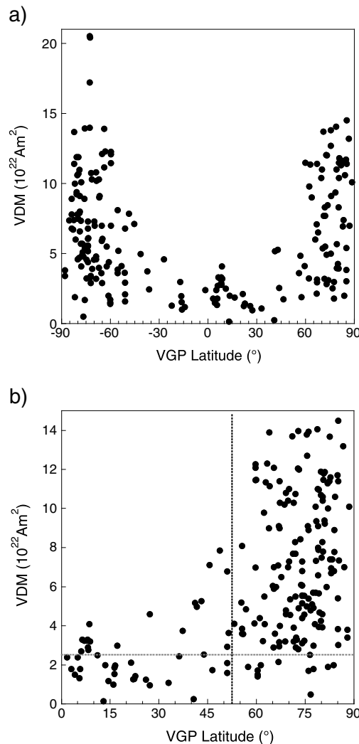
Figure 9. (a) Virtual dipole moments as a function of VGP latitude from volcanic reversal records for which absolute paleointensity determinations are available. (b) Same as Figure 9a after reversing the negative VGP latitudes.
