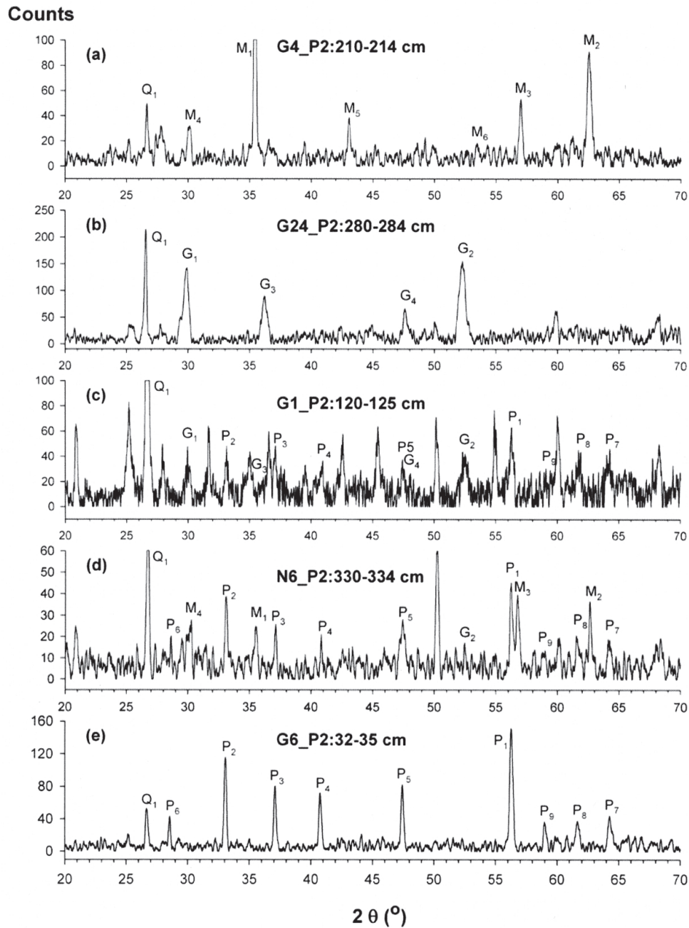
Fig. 4. Representative X-ray diffraction data for magnetic extracts from the intervals of the studied piston cores. The main peaks for magnetite (M 1 - M 6 ), greigite (G 1 - G 4 ), pyrite (P 1 - P 9 ) and Quartz (Q 1 ) are shown. Peak intensities that are over-scale have been cut.
